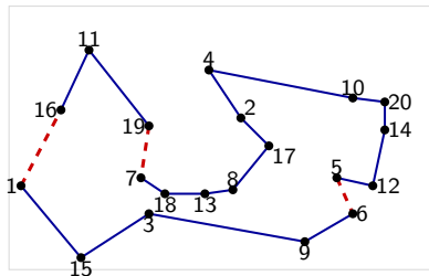
(a) local optimum: L = 319
