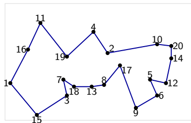
(c) after 2-opt: L = 303
