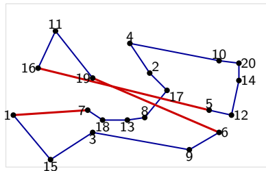
(b) after the double bridge: L = 432
