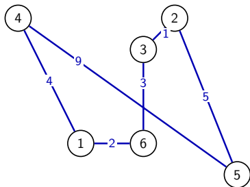
multi-start NN (from city 2): L = 24
