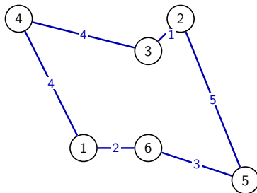
FI from city 1: L = 19 = z(I)
