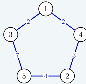
optimal tour: L = 18
