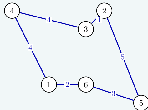
FI from city 1: L = 19 = z(I)
