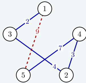
NN from city 1: L = 25 (dashed: the closing edge)
