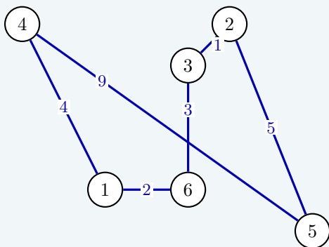
multi-start NN (from city 2): L = 24
